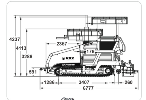
EXTERIOR DRAWING
