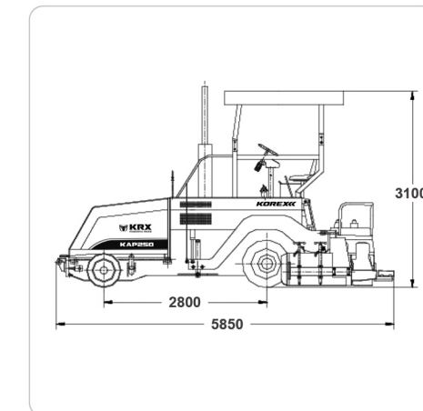
EXTERIOR DRAWING
