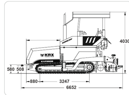
EXTERIOR DRAWING
