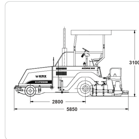
EXTERIOR DRAWING
