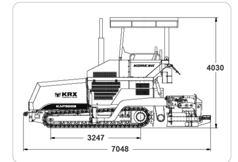
EXTERIOR DRAWING
